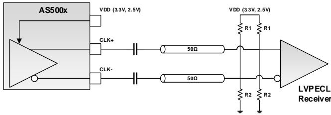
AC-Coupled Self-Biased LVPECL - Thevenin Termination
