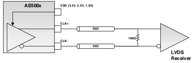
DC-Coupled LVDS
